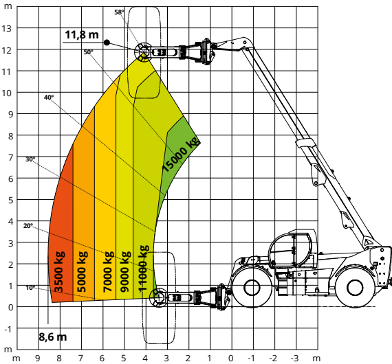
LOAD CHART WITH TYRES CLAMP MODEL TC 16.63
